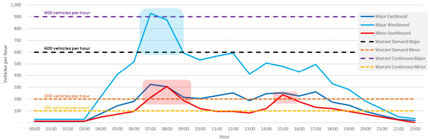
Figure 2.1 East-West Sub-Arterial Road and Road 14 (School Road) – comparison of forecast traffic volumes to traffic signal warrants
