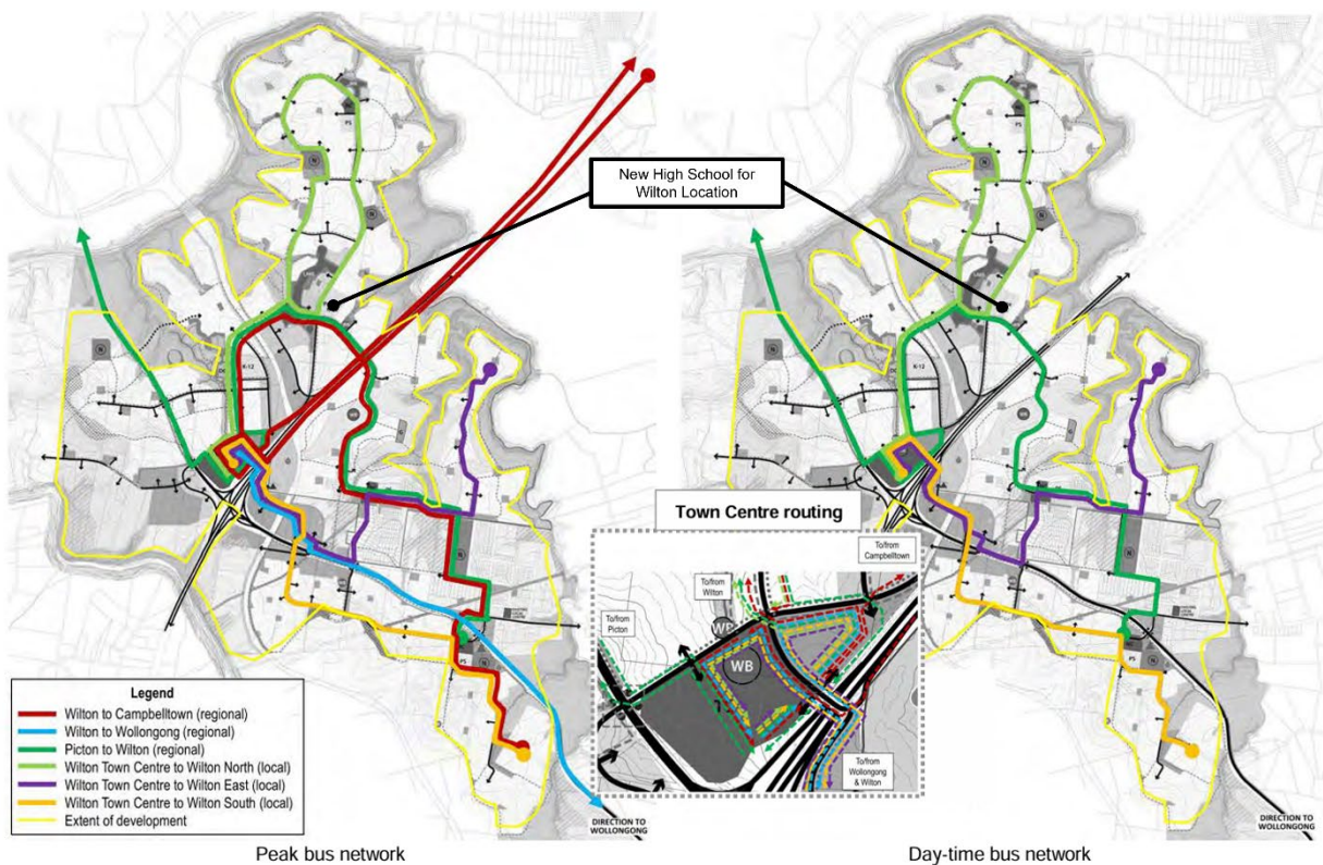
Figure 9: Proposed Bus Network for Wilton Junction Full Development 8
