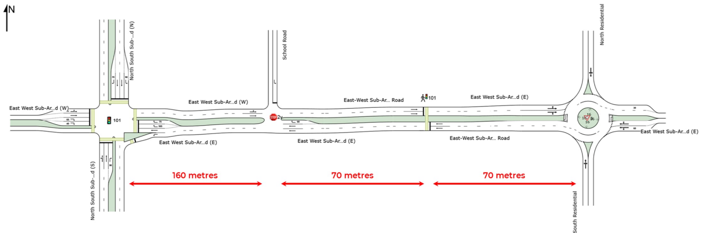
Figure 1.1 Intersection spacing along East-West Sub-arterial Road
